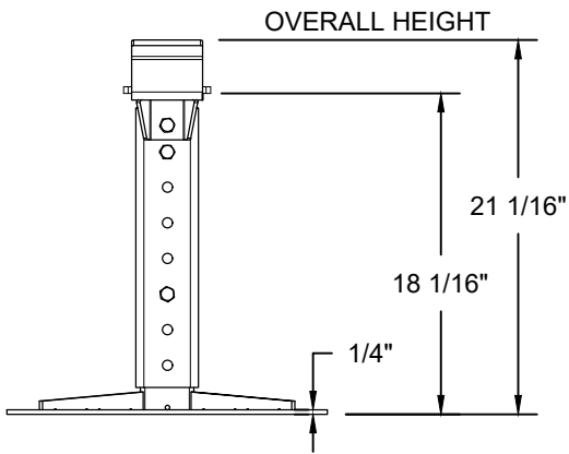
FULLY RETRACTED
