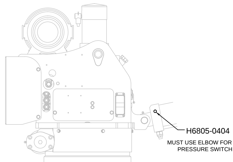
RIGHT SIDE
