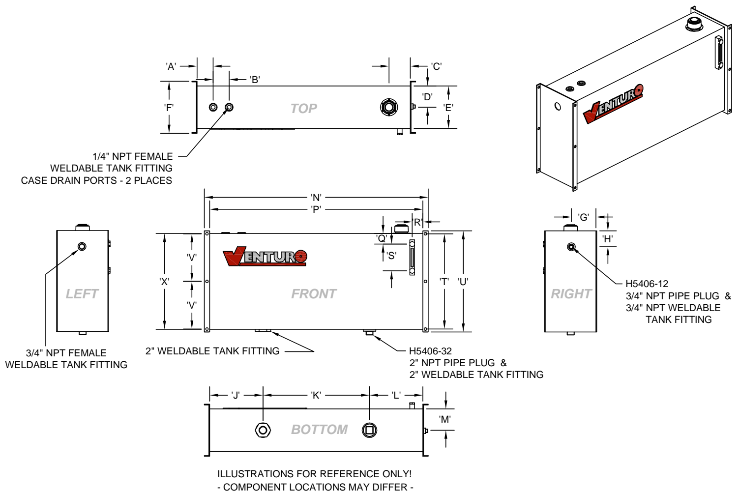
HYD. TANK DIMENSION (HTD) CHART
