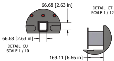
HITCH WITH RECEIVER TUBE
