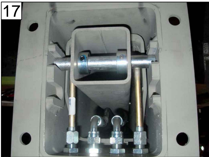
WITH CYLINDER HOUSING CENTERED LOCTITE & FASTEN COLLARS FLUSH
