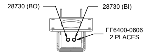
SECTION VIEW B-B 16' BOOM
