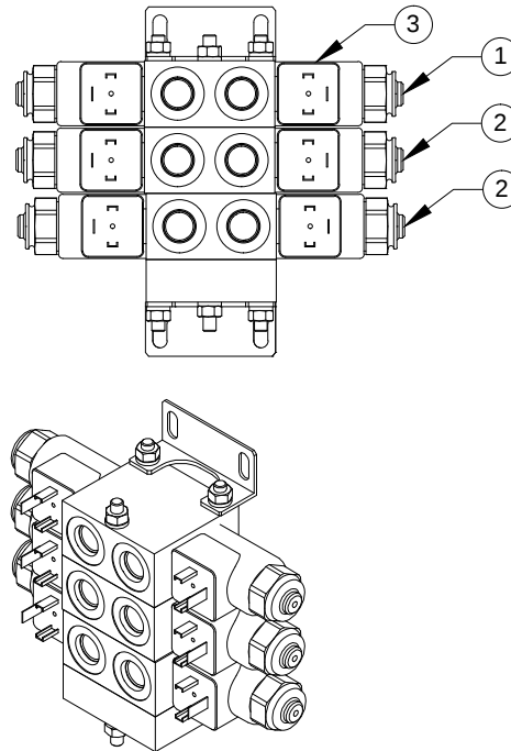
28801 3-SPOOL NON-PROPORTIONAL
