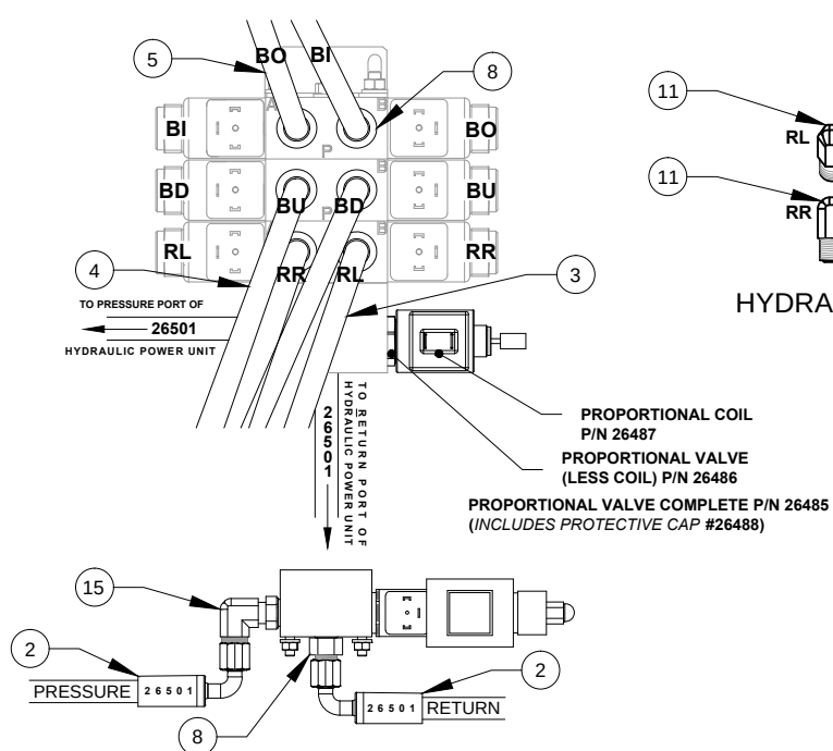
PROPORTIONAL VALVE BLOCK
