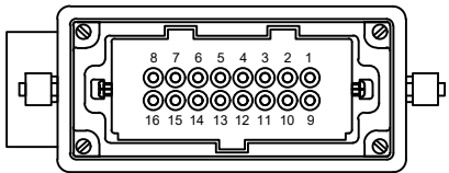
VIEW FROM CONNECTING FACE
