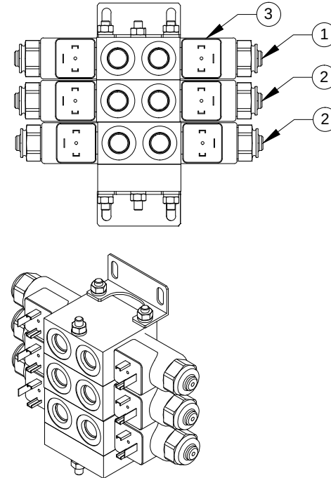
28801 3-SPOOL NON-PROPORTIONAL
