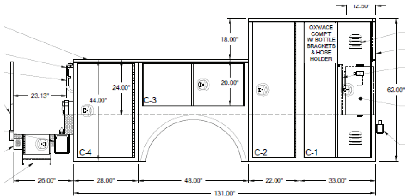
CURB SIDE VIEW
