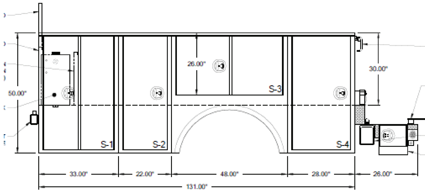
STREET SIDE VIEW
