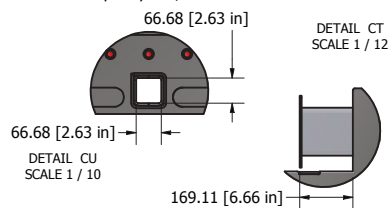
HITCH WITH RECEIVER TUBE
